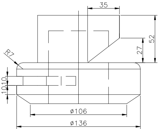
FRONT SCALE 1/2
