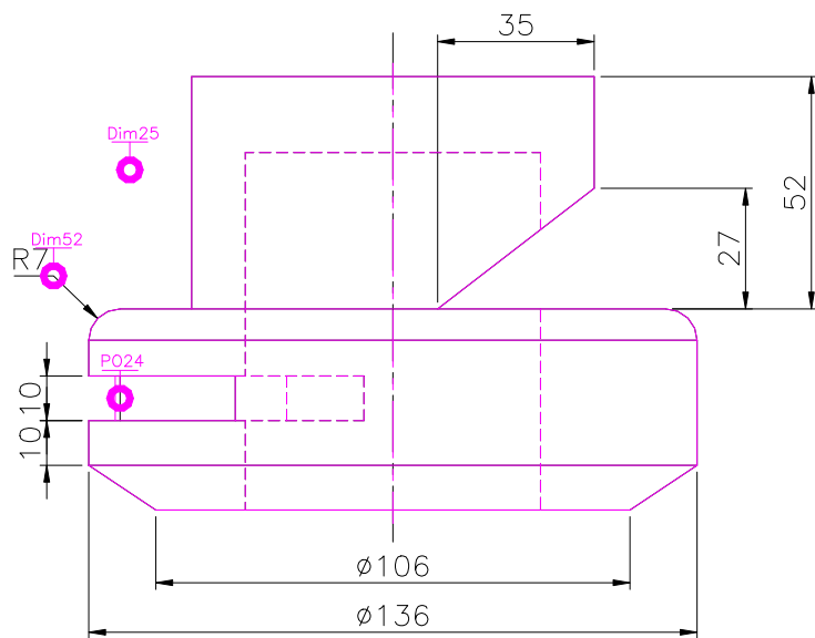
FRONT SCALE 1/2
