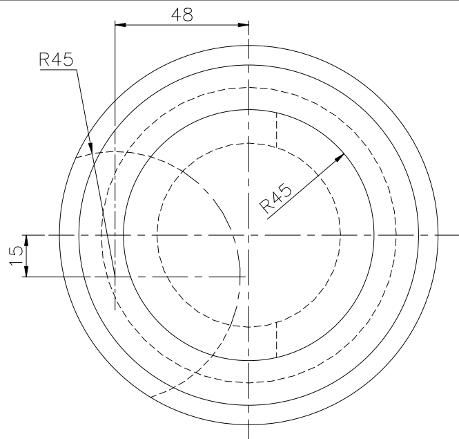
TOP SCALE 1/2
