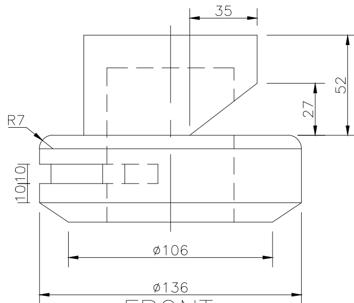
FRONT SCALE 1/2
