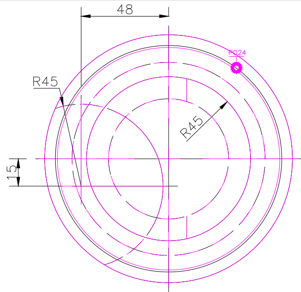
TOP SCALE 1/2
