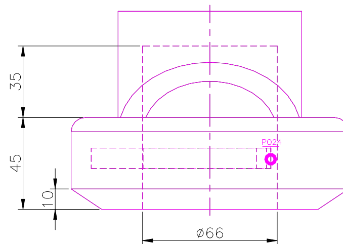
RIGHT SCALE 1/2
