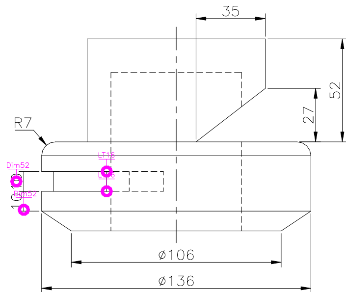
FRONT SCALE 1/2
