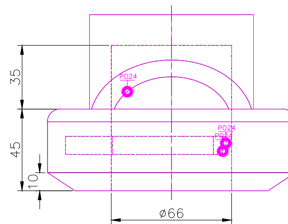
RIGHT SCALE 1/2
