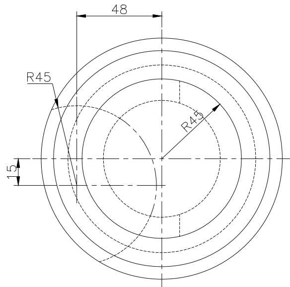
TOP SCALE 1/2
