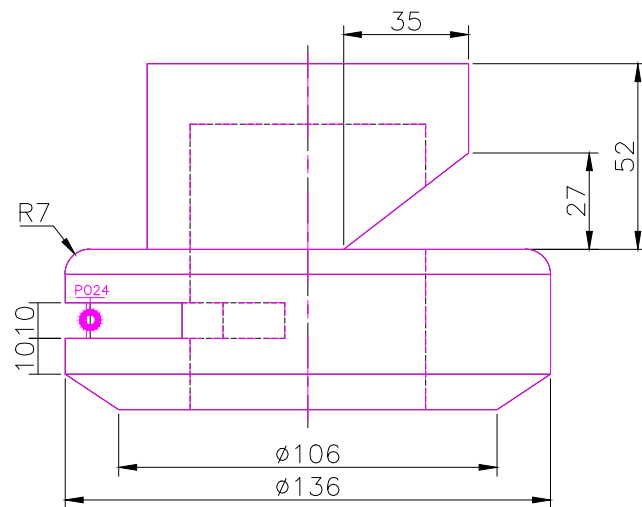
FRONT SCALE 1/2
