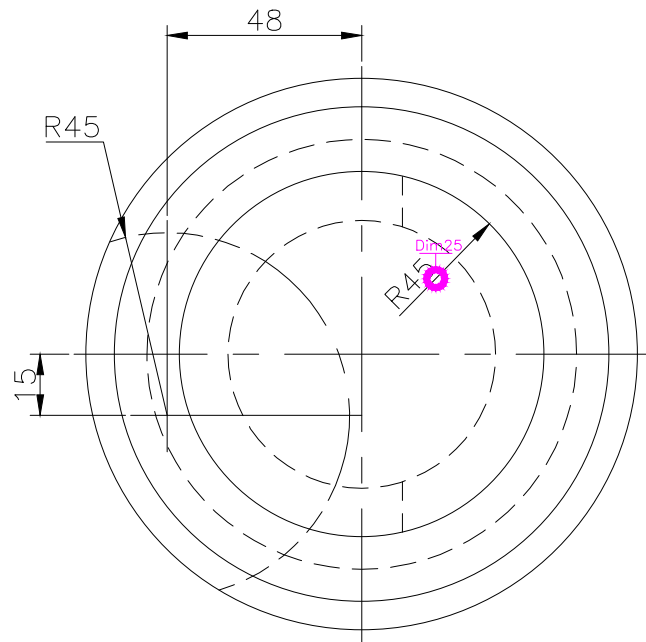
TOP SCALE 1/2
