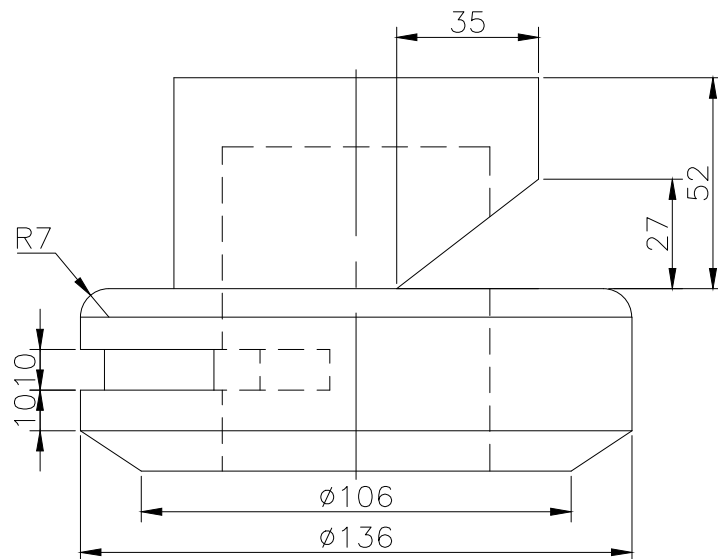
FRONT SCALE 1/2
