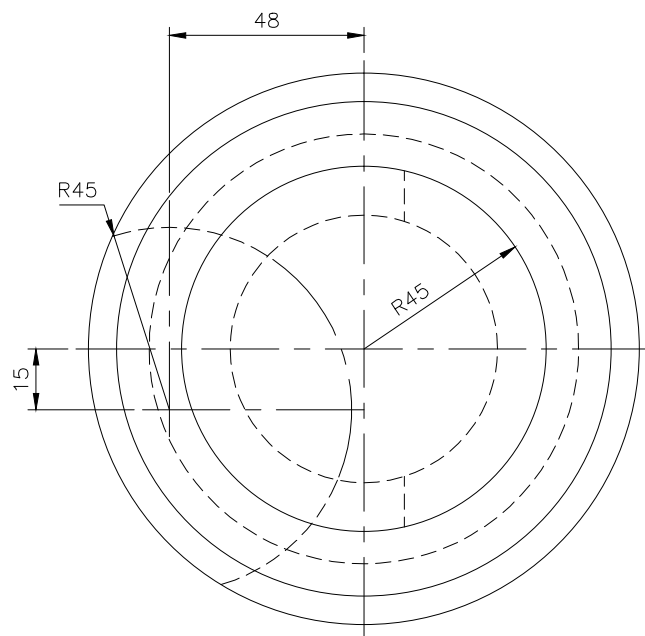
TOP SCALE 1/2
