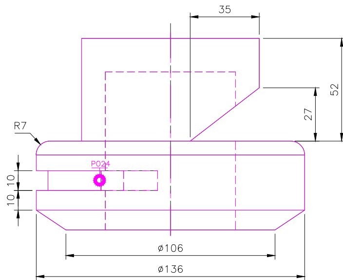
FRONT SCALE 1/2
