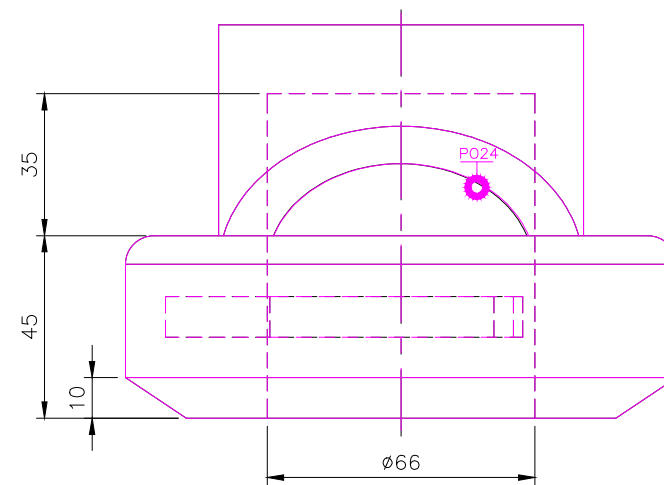
RIGHT SCALE 1/2
