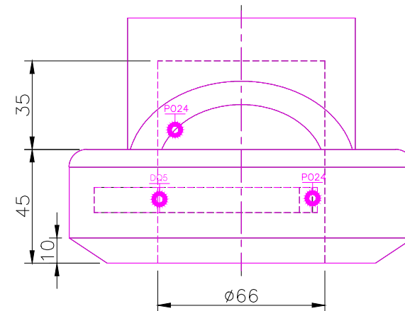
RIGHT SCALE 1/2
