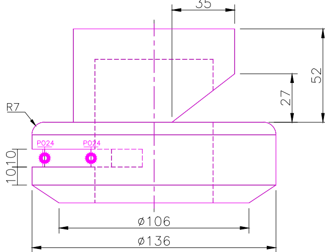
FRONT SCALE 1/2
