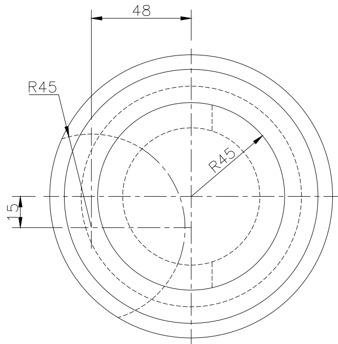
TOP SCALE 1/2
