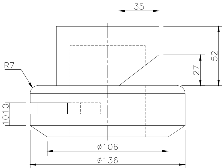
FRONT SCALE 1/2
