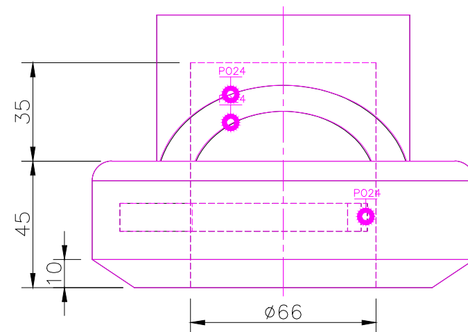
RIGHT SCALE 1/2
