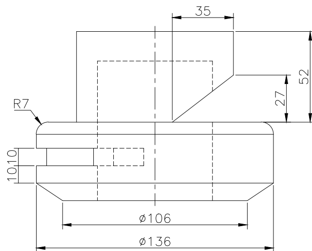
FRONT SCALE 1/2
