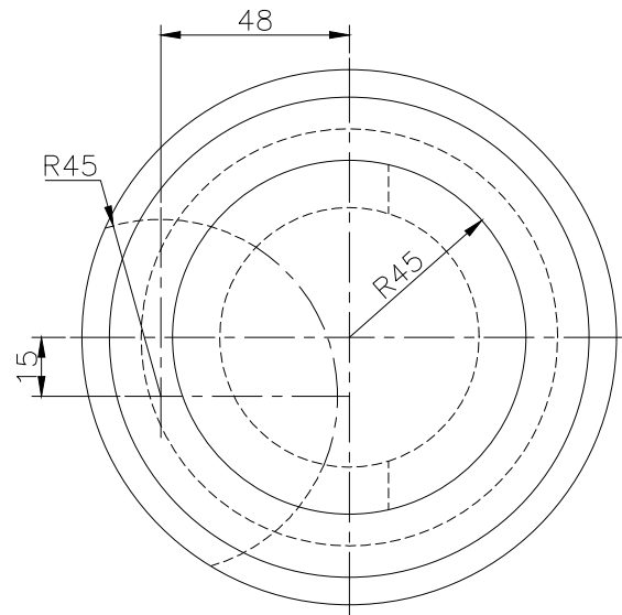
TOP SCALE 1/2
