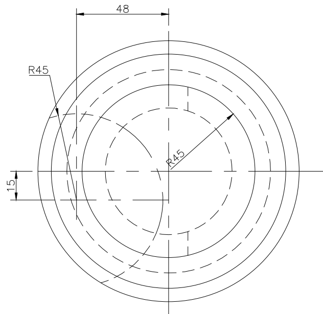
TOP SCALE 1/2
