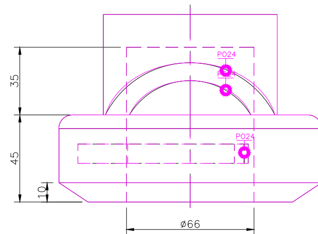
RIGHT SCALE 1/2
