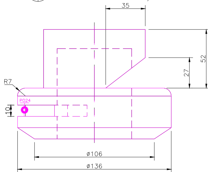
FRONT SCALE 1/2
