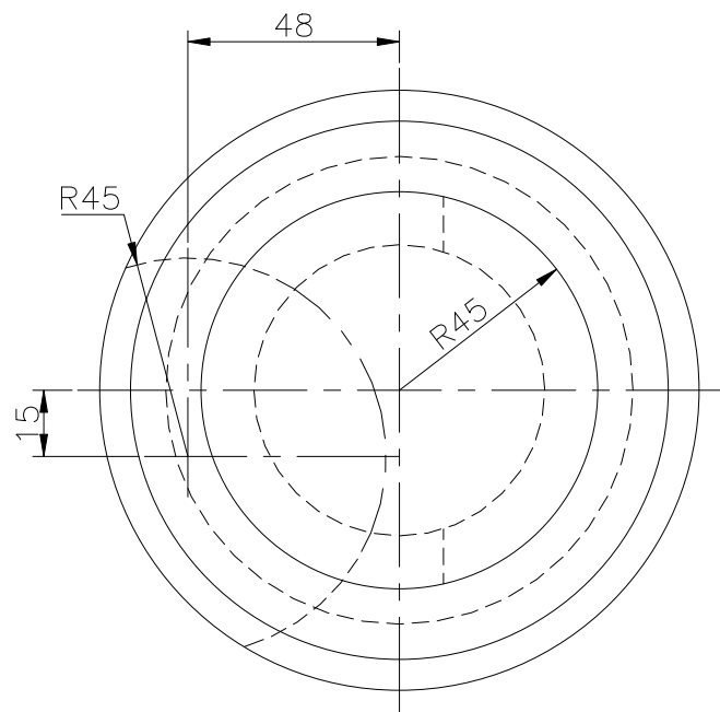
TOP SCALE 1/2
