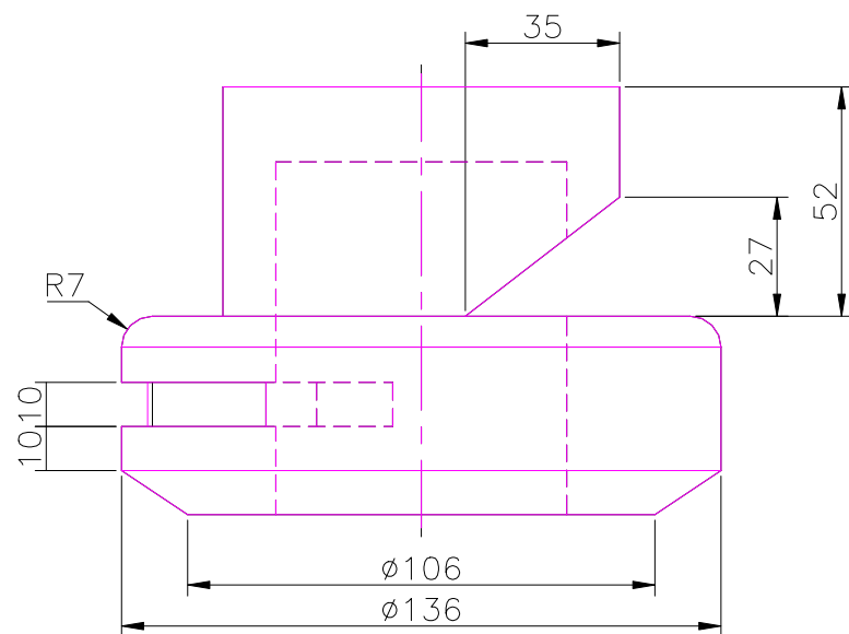
FRONT SCALE 1/2
