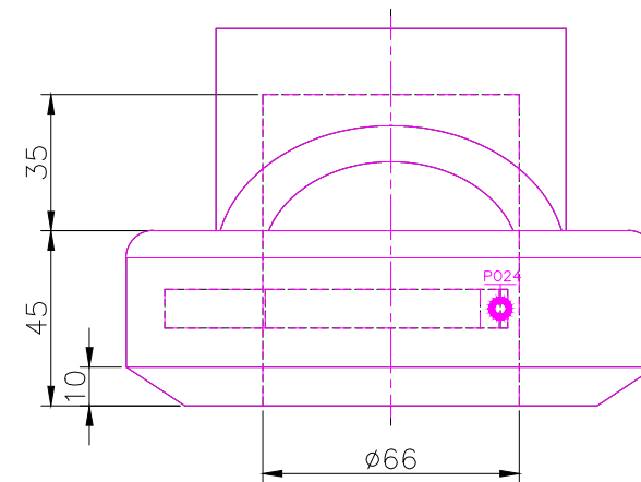
RIGHT SCALE 1/2
