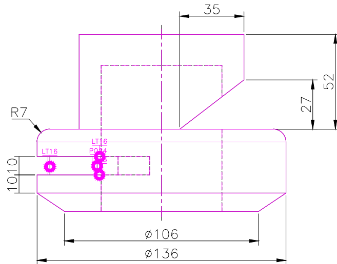
FRONT SCALE 1/2
