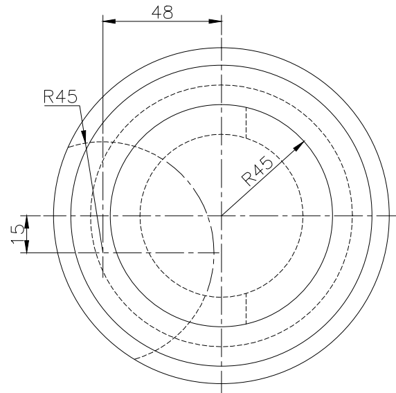
TOP SCALE 1/2
