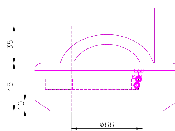
RIGHT SCALE 1/2
