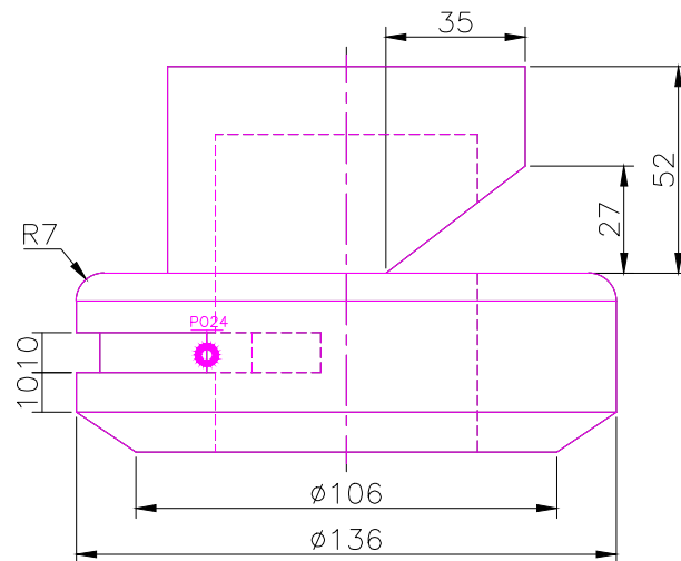
FRONT SCALE 1/2
