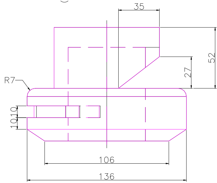
FRONT SCALE 1/2
