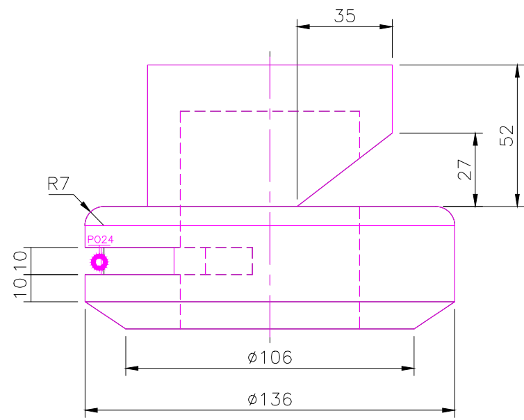
FRONT SCALE 1/2
