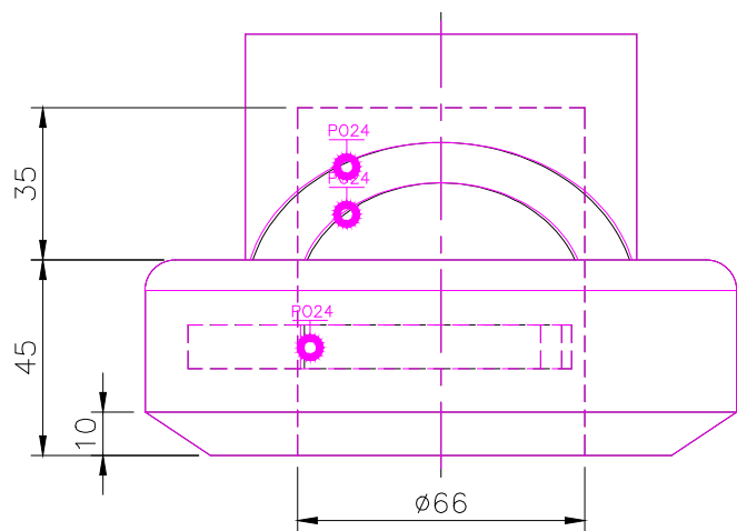
RIGHT SCALE 1/2
