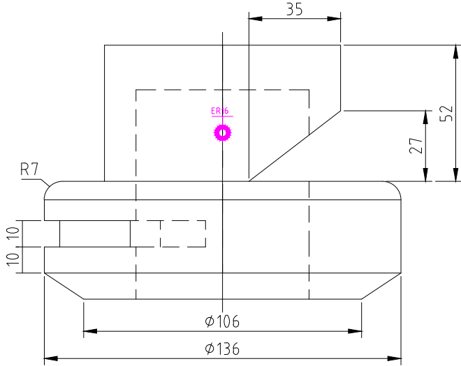
FRONT SCLAE 1/2
