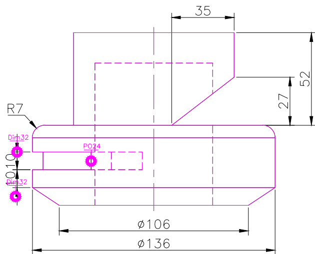
FRONT SCALE 1/2
