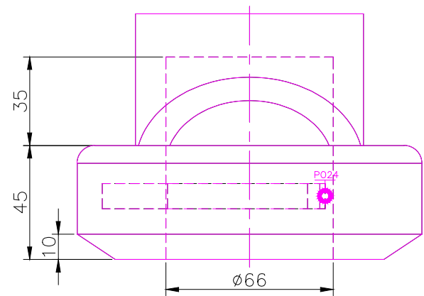
RIGHT SCALE 1/2
