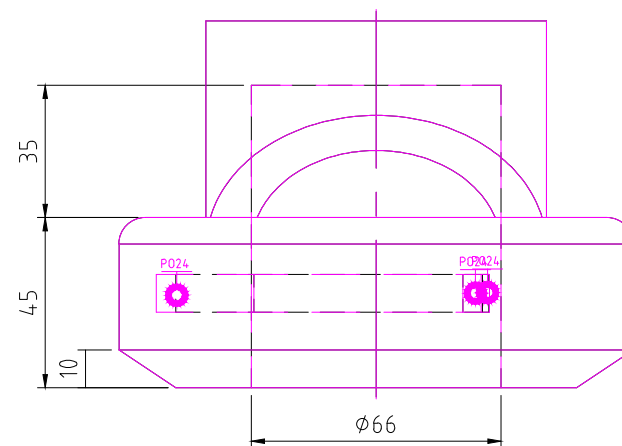
RIGHT SCALE 1/2
