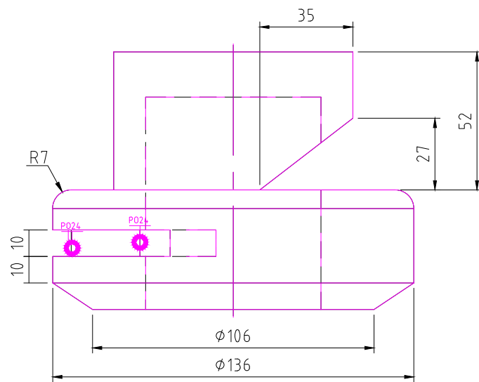
FRONT SCALE 1/2
