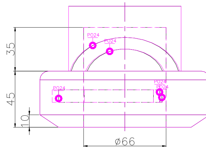
RIGHT SCALE 1/2
