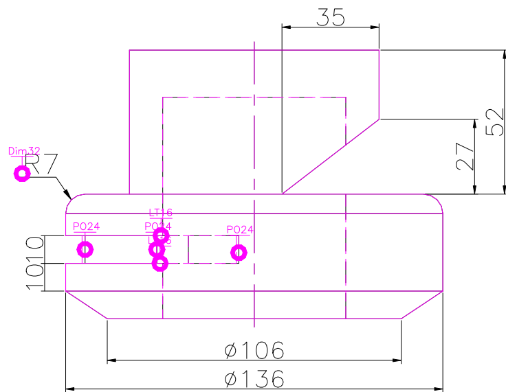
FRONT SCALE 1/2
