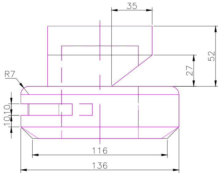
TOP SCALE 1/2
