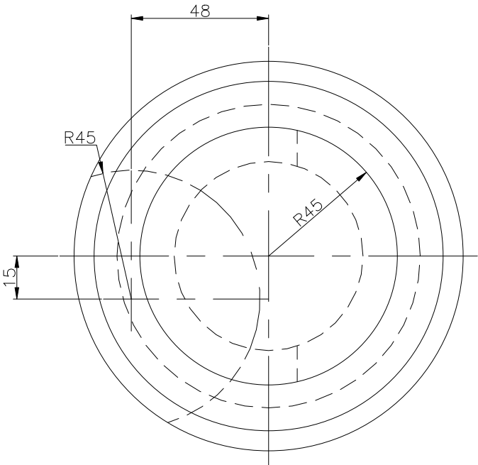
TOP SCALE 1/2
