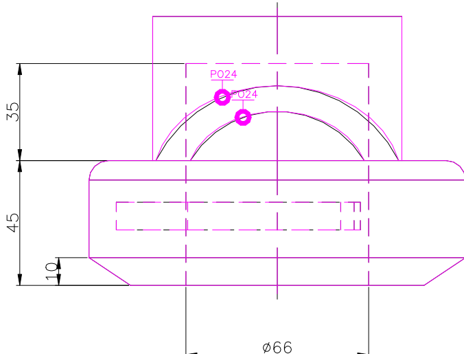
RIGHT SCALE 1/2
