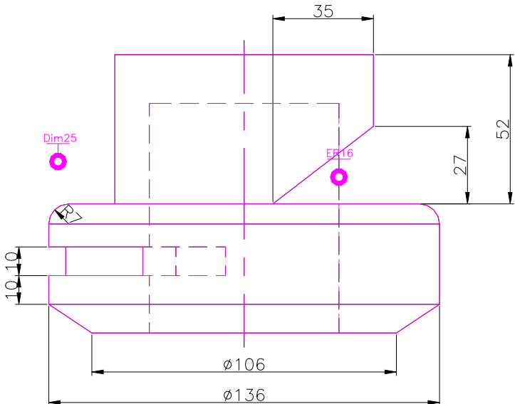
FRONT SCALE 1/2
