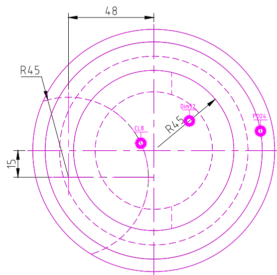
TOP SCALE 1/2
