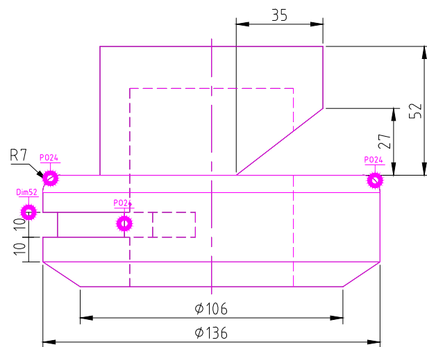
FRONT SCALE 1/2
