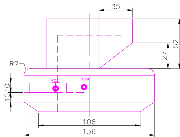
FRONT SCALE 1/2
