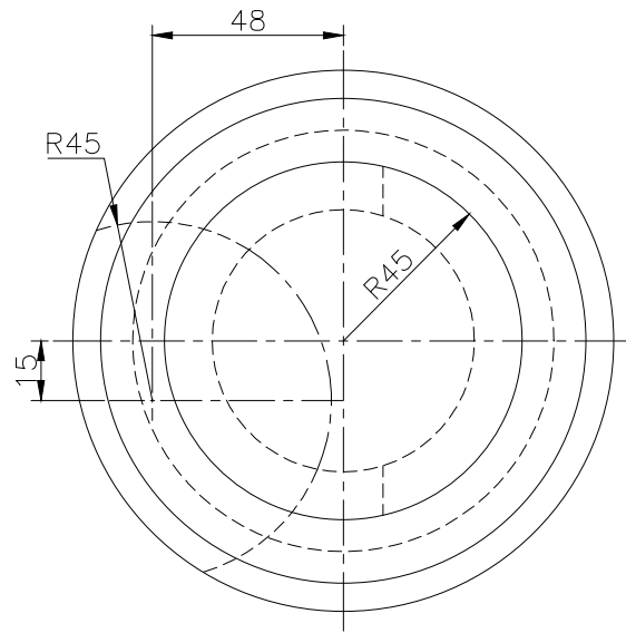
TOP SCALE 1/2
