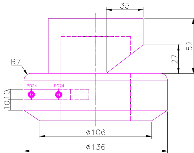
FRONT SCALE 1/2
