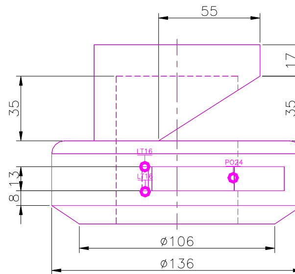
RIGHT SCALE 1/2
