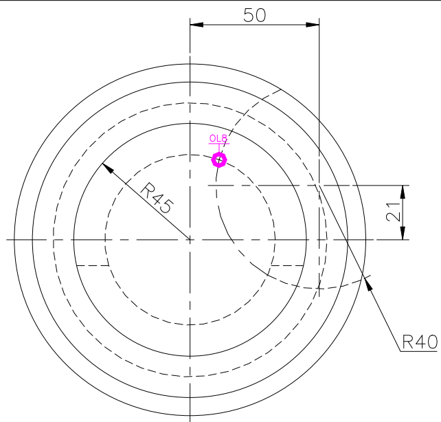
TOP SCALE 1/2
