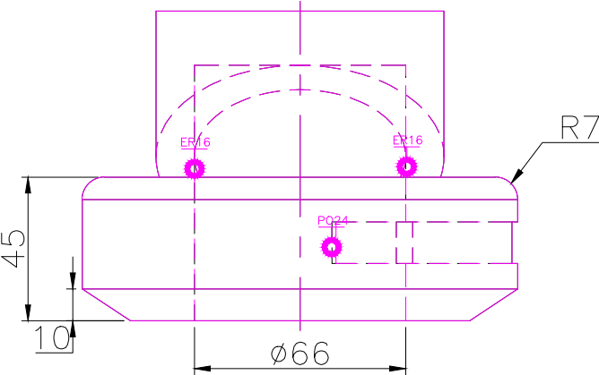
FRONT SCALE 1/2
