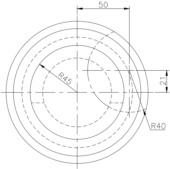
TOP SCALE 1/2
