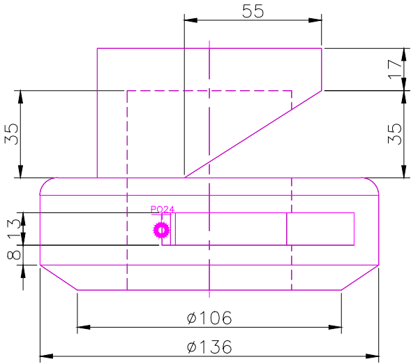
RIGHT SCALE 1/2
