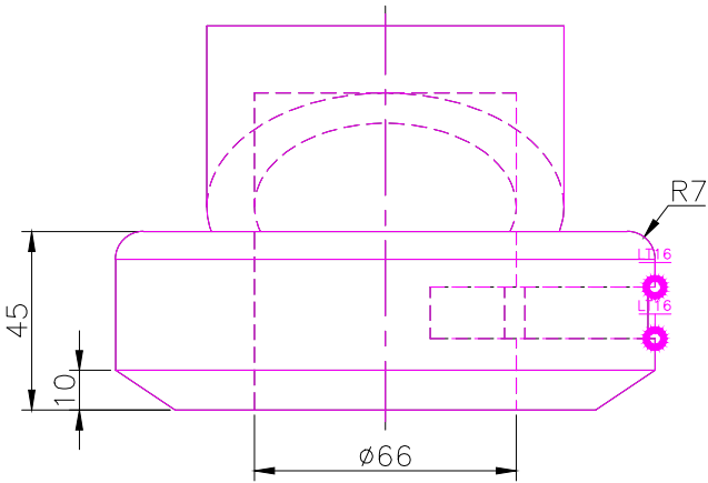
FRONT SCALE 1/2
