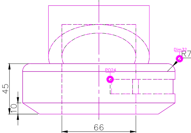
FRONT SCALE 1/2
