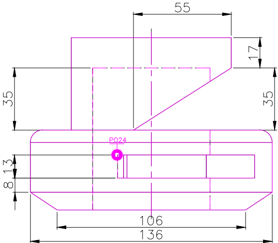
RIGHT SCALE 1/2
