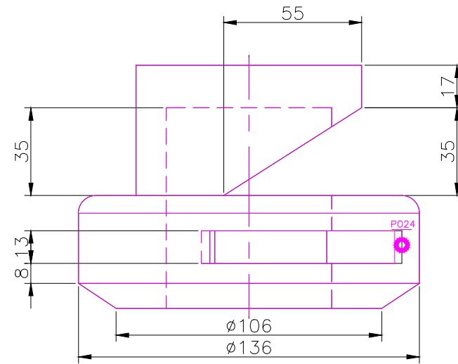
RIGHT SCALE 1/2
