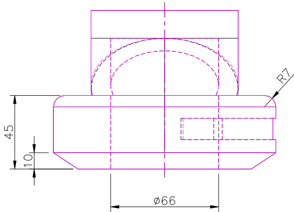
Top View SCALE 1/2
