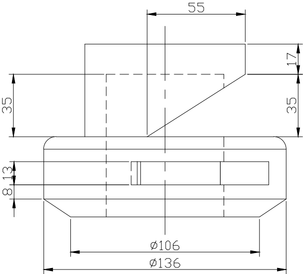
RIGHT SCALE 1/2
