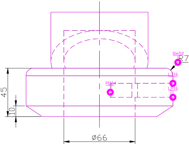
FRONT SCALE 1/2
