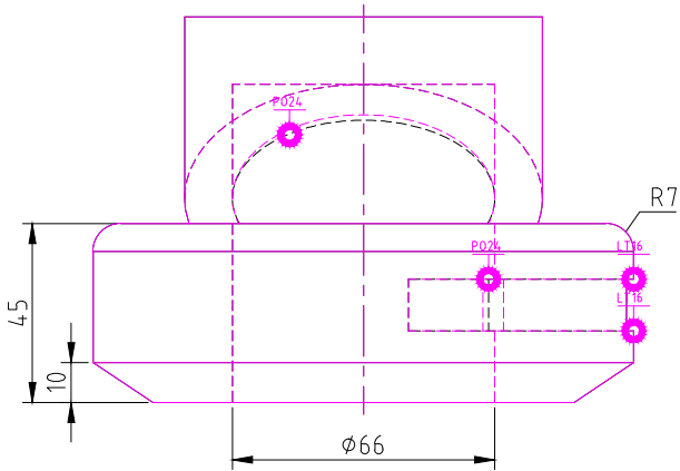
FRONT SCALE 1/2
