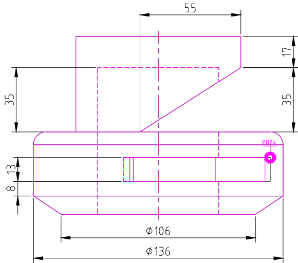
RIGHT SCALE 1/2
