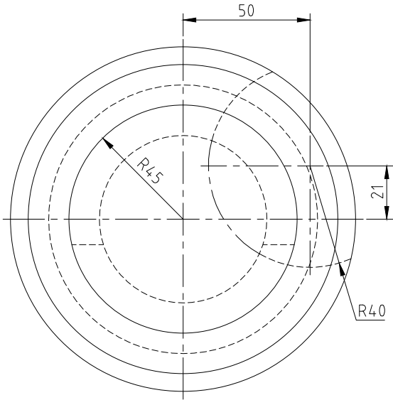
TOP SCALE 1/2
