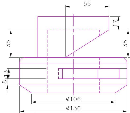
RIGHT SCALE 1/2
