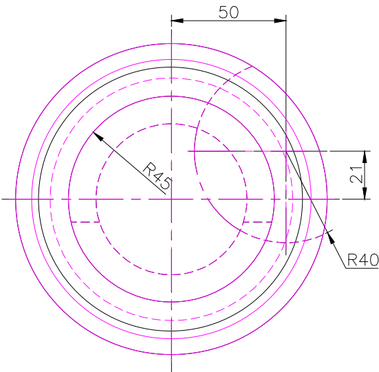
TOP SCALE 1/2
