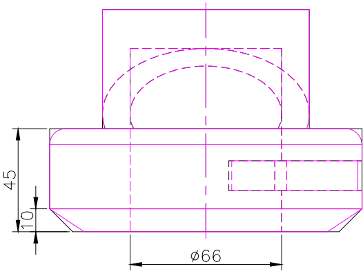
FRONT SCALE 1/2
