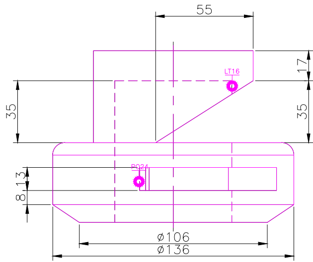
RIGHT SCALE 1/2
