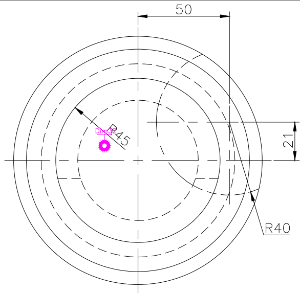
TOP SCALE 1/2
