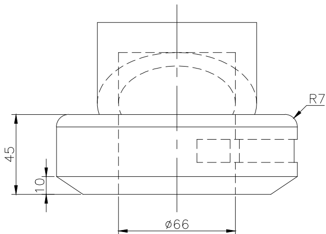
FRONT SCALE 1/2
