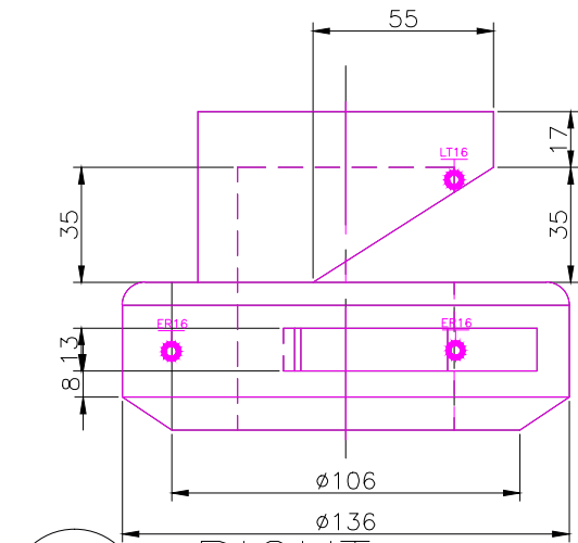
RIGHT SCALE 1/2
