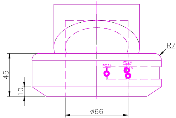
FRONT SCALE 1/2
