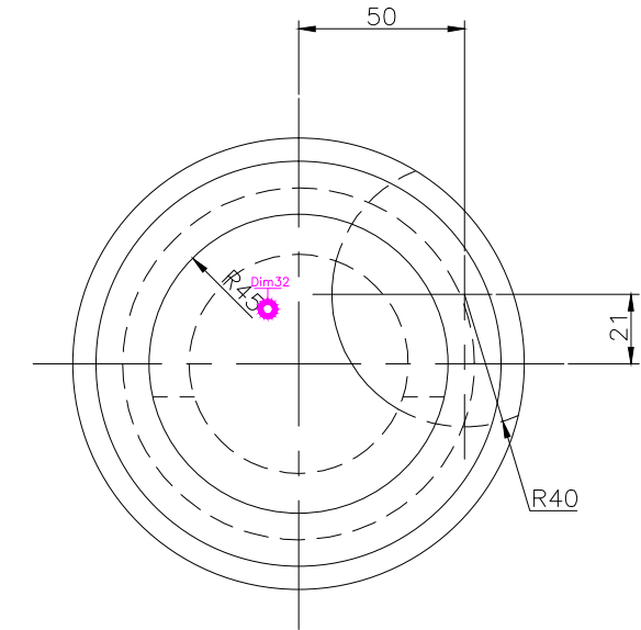
TOP SCALE 1/2
