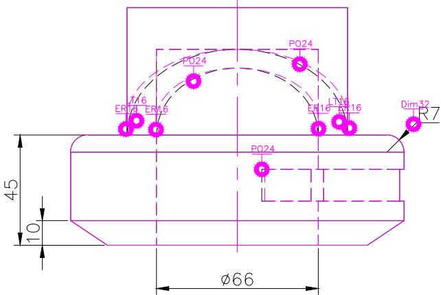
FRONT SCALE 1/2
