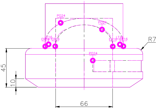
FRONT SCALE 1/2
