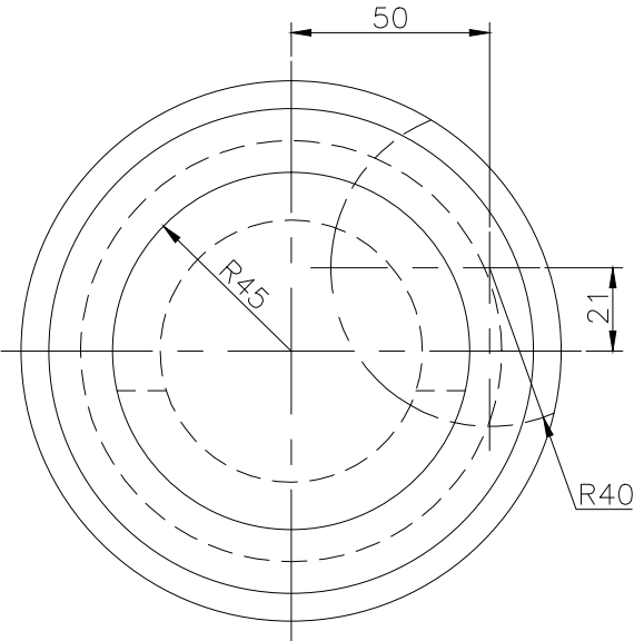
TOP SCALE 1/2
