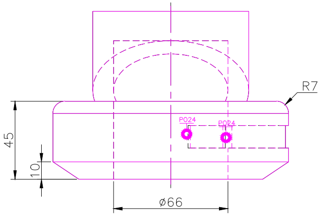
FRONT SCALE 1/2
