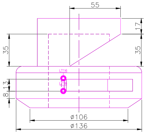
RIGHT SCALE 1/2
