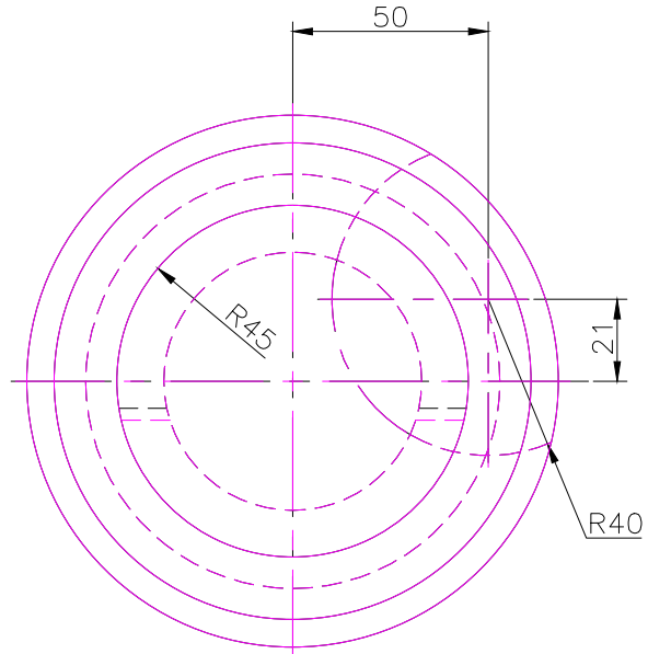
TOP SCALE 1/2
