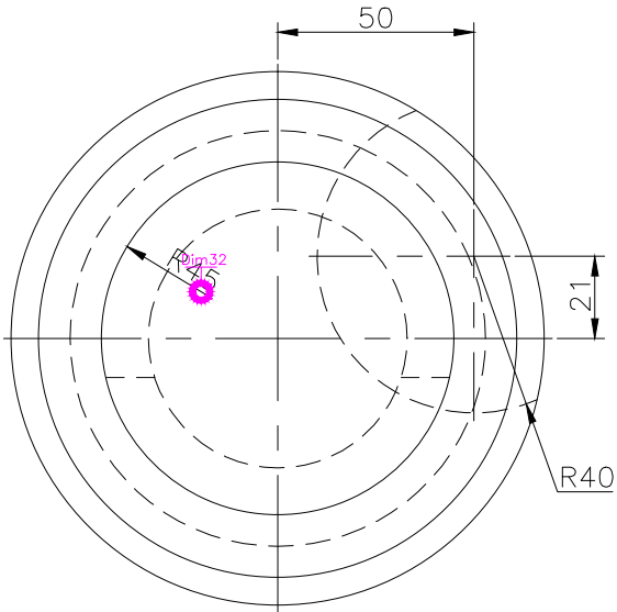
TOP SCALE 1/2
