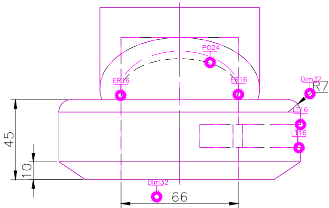
FRONT SCALE 1/2
