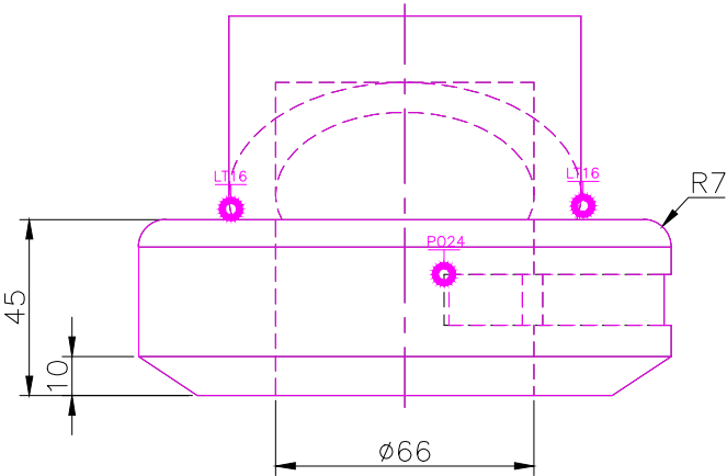
FRONT SCALE 1/2
