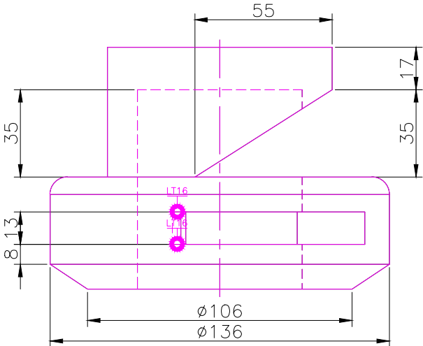
RIGHT SCALE 1/2
