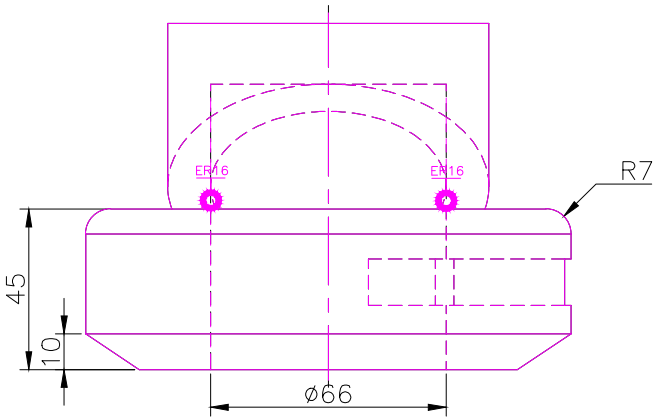
FRONT SCALE 1/2
