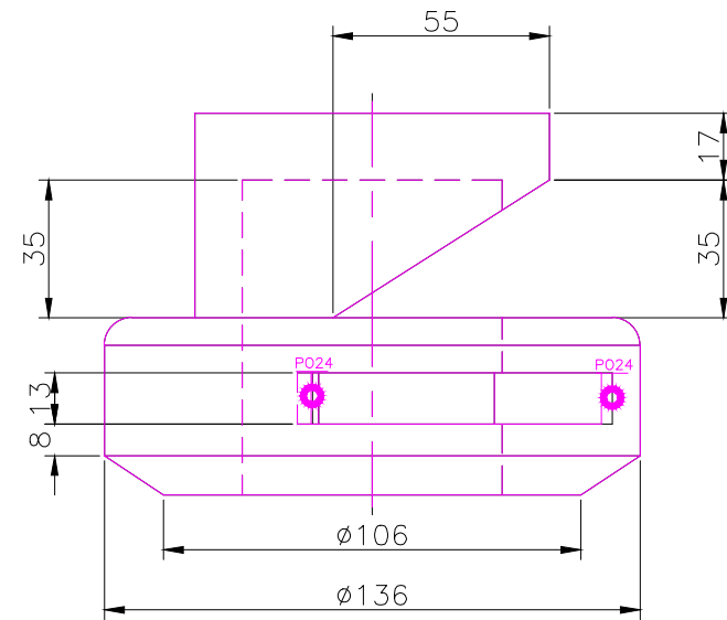
RIGHT SCALE 1/2
