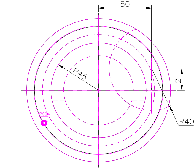
TOP SCALE 1/2
