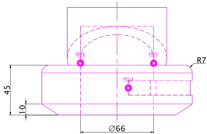
FRONT SCALE 1/2
