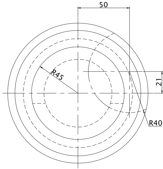
TOP SCALE 1/2
