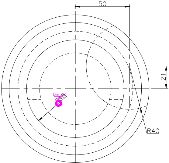
TOP SCALE 1/2
