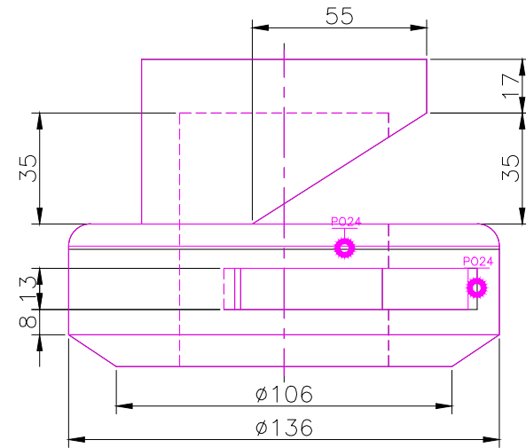
RIGHT SCALE 1/2
