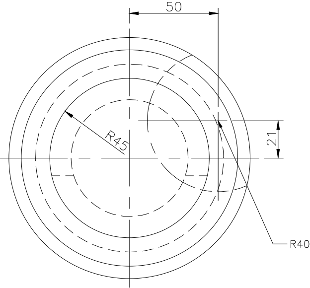
TOP SCALE 1/2
