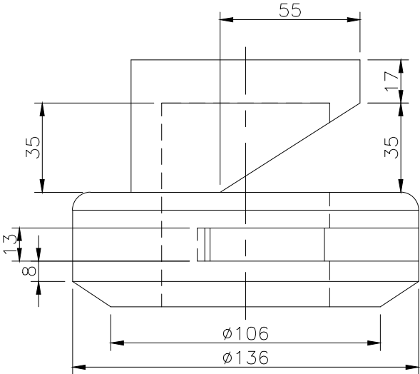
RIGHT SCALE 1/2
