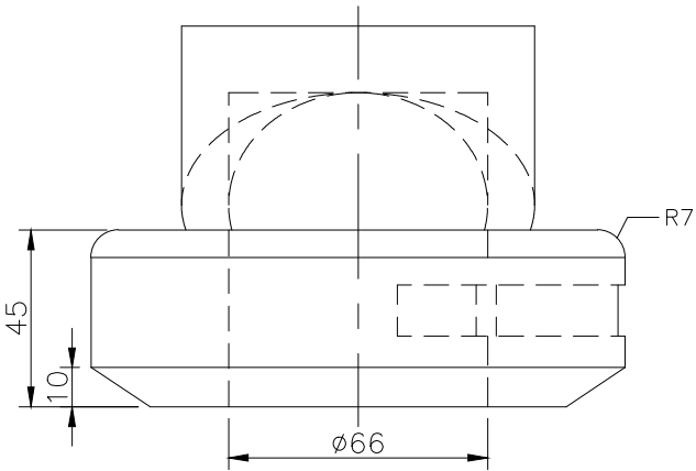
FRONT SCALE 1/2
